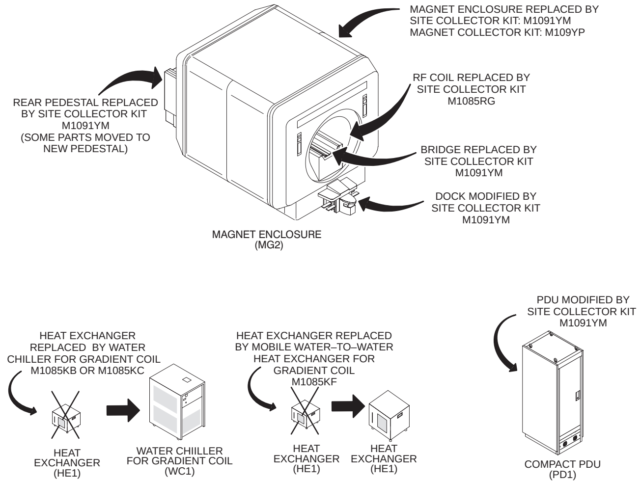
SIGNA CVMR SYSTEM WITH LCC MAGNET EXISTING HARDWARE REPLACED OR MODIFIED & NEW EQUIPMENT ADDED ILLUSTRATION 1-3
